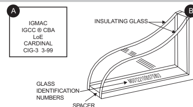
Markings are etched in the glass (A) or are printed/stamped on one of the four sides of the spacer channel which separates the two panes of glass (B).
